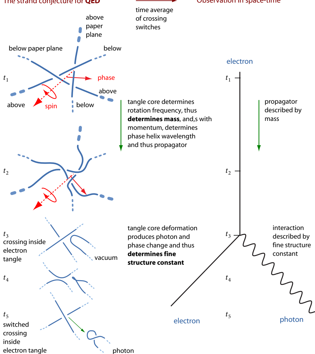
FIGURE 74 QED in one picture: In the strand model, the electron mass and the fine structure constant are determined by the tangle – only the simplest family member is shown here – and its shape change under fluctuations.
